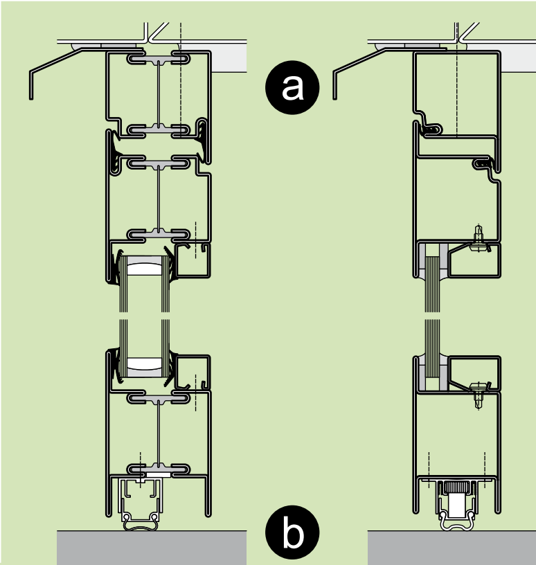
Typical open out door with thermal barrier
